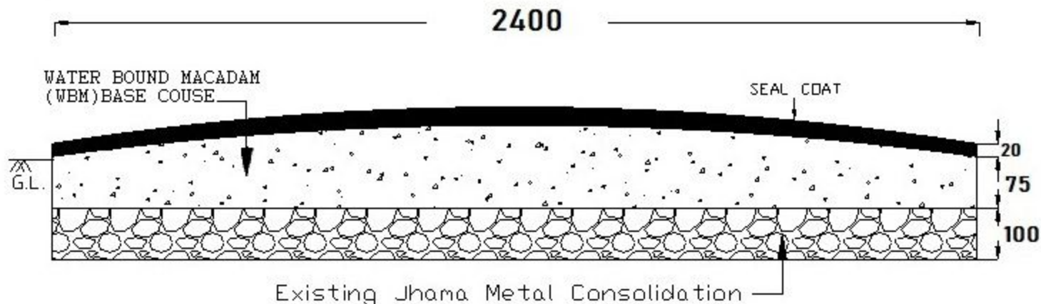
CROSS-SECTION OF LOW-VOLUME BITUMINOUS ROAD
