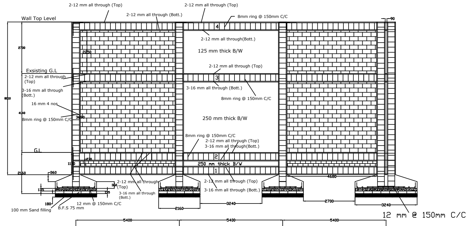
SECTIONAL ELEVATION
