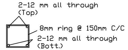
Beam 4 - (250x250)
