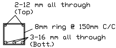
Beam 1,2,3 - (250x250)
